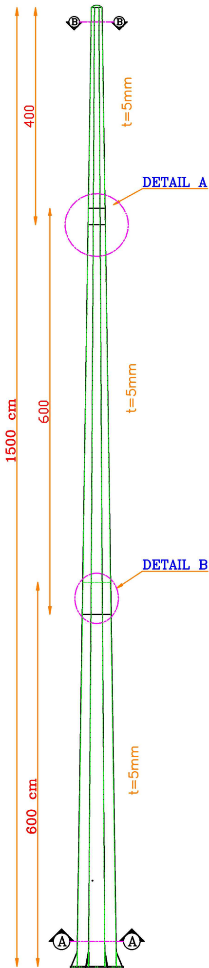
t=5mm Sec: AA
